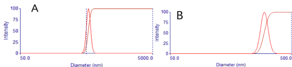
Figure 1: Size distribution of (A) Rh-silica; (B) Eggshell-Calcium Carbonate
