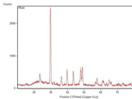
Figure 5: X-ray diffraction spectra of coated zirconia
